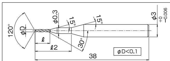
\ell 2 = 2.0 \phi D = \phi 0.03 \sim \phi 0.04 \ell 2 = 3.0 \phi D = \phi 0.05 \sim \phi 0.09
